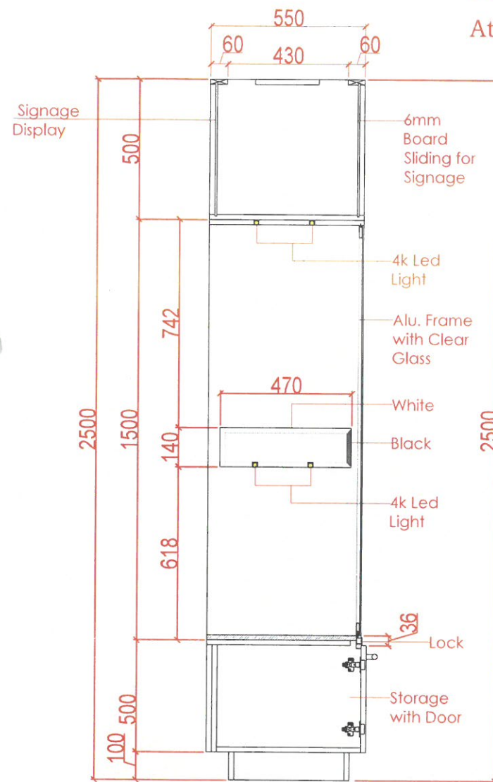
Sectional Details
